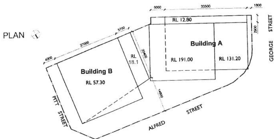
FIGURE 2.69 - 1 Alfred Street Site Development Control Envelope
